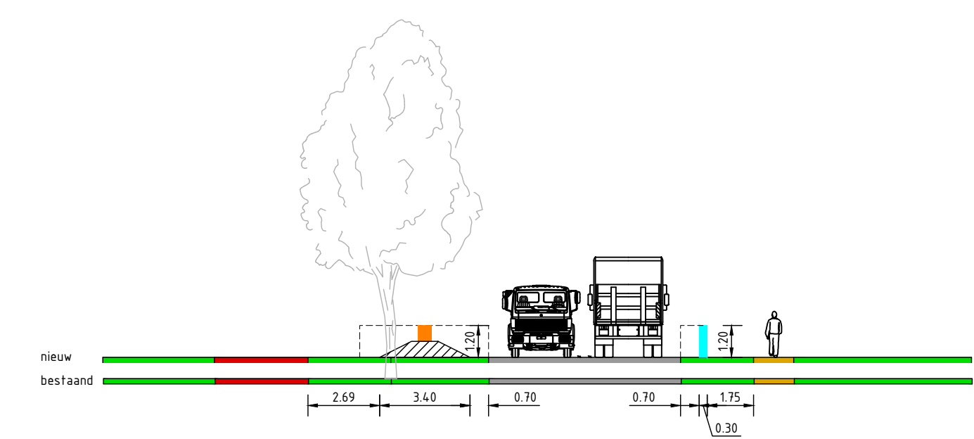
PRINCIPEPROFIEL 4-4 VARIANT 3
